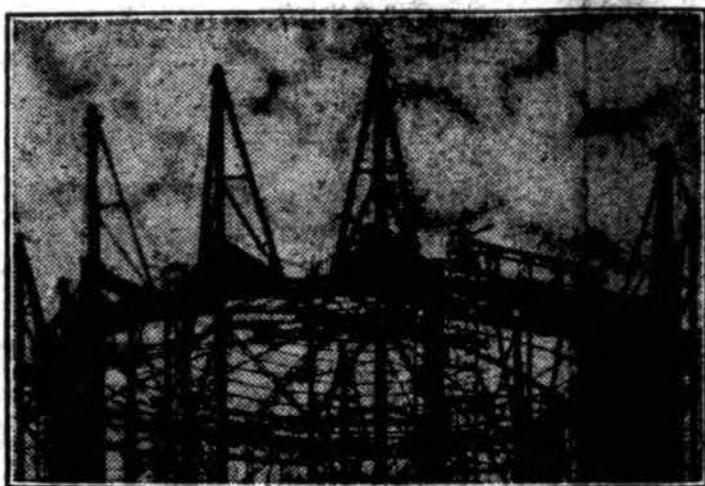
Great Dome of Travel & Transport Building of Century of Progress nearing completion. Construction features never before used make it an engineering wonder.
