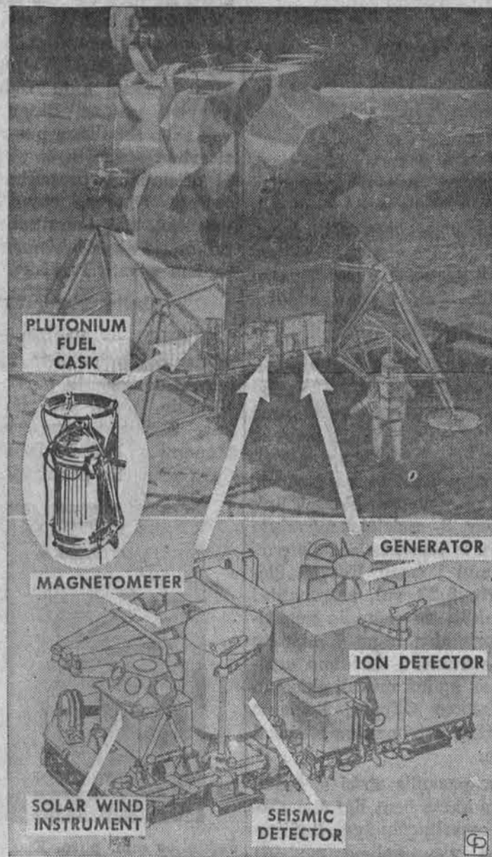
LUNAR MODULE SCIENTIFIC BAY — This illustration shows (top) Quad 2, the Lunar Module's scientific equipment bay for experiment packages (closeup bottom). Tools and collecting equipment are in Quad 4 on the opposite side.
